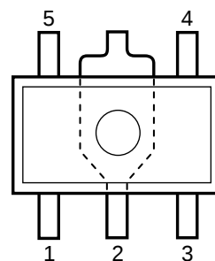
RP511H (SOT-89-5) Pin Configuration
