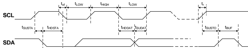
Figure 17. I2C / SMBus Timing
