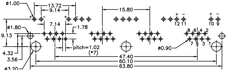
PC Board Layout(t=1.60mm) Component Side Shown
