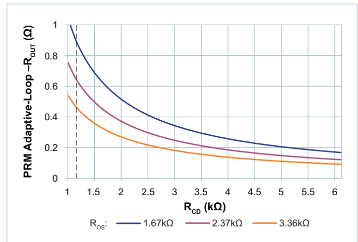
Figure 25 — Programming the adaptive-loop compensation with R_{\text{VC}} = 1\text{k}\Omega
