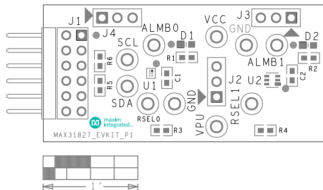
MAX31827 EV System Component Placement Guide—Top Silkscreen
