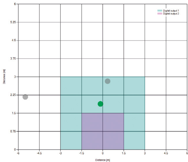
Figure 14: Default detection areas for digital outputs
