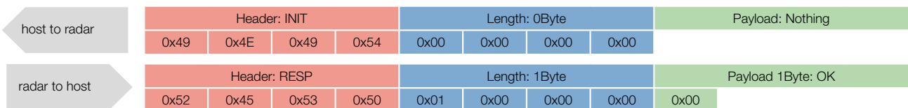
Figure 15: Example INIT command
