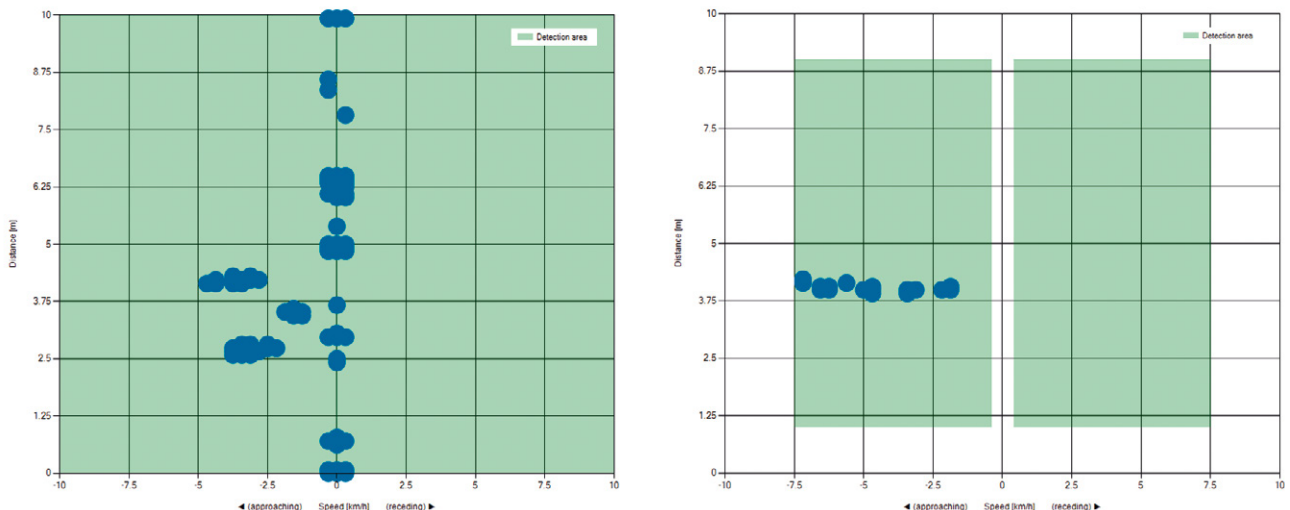
Figure 12: Influence of distance and speed limitation to raw targets
