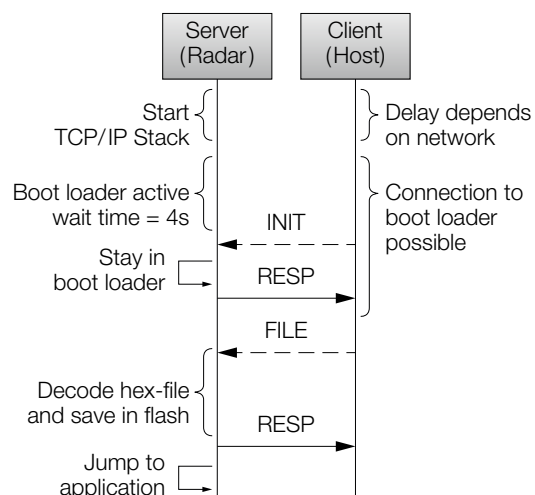
Figure 22: Start-up with connection to boot loader and firmware update
