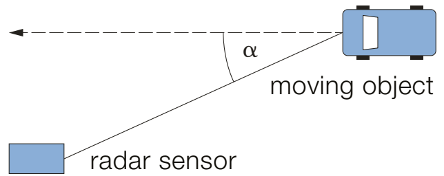
Figure 7: Tangential speed compensation
