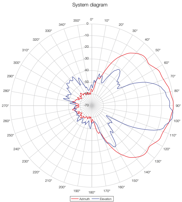
Figure 2: Antenna characteristics
