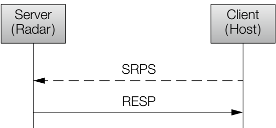
Figure 25: Set parameter structure
