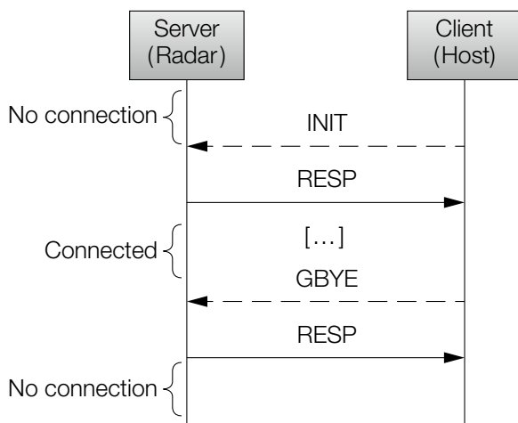
Figure 20: Connection
