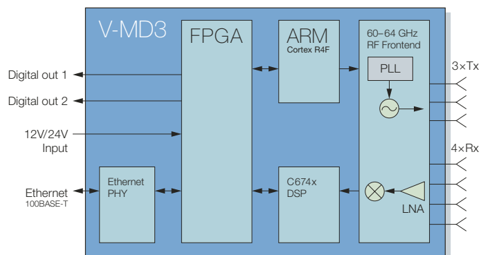
Figure 1: block diagram
