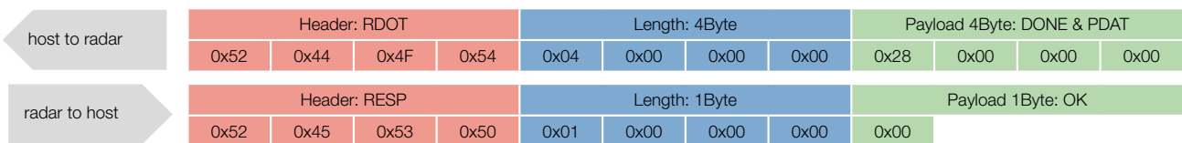
Figure 16: Example RDOT command
