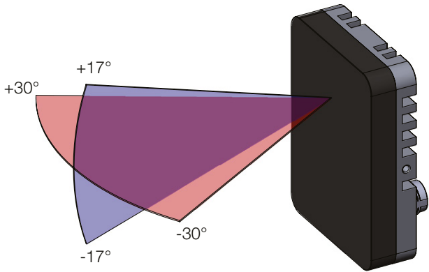
Figure 3: Antenna orientation
