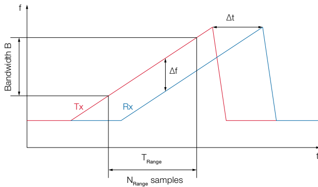
Figure 5: FMCW TX and RX chirp example
