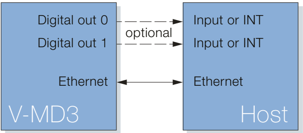
Figure 10: Host driven connection example
