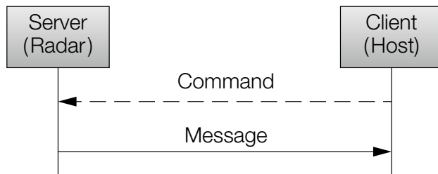
Figure 18: Client-Server model
