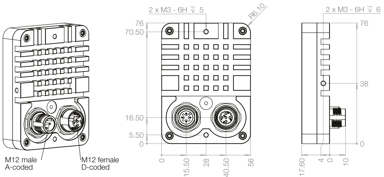
Figure 26: Outline dimensions in millimetre
