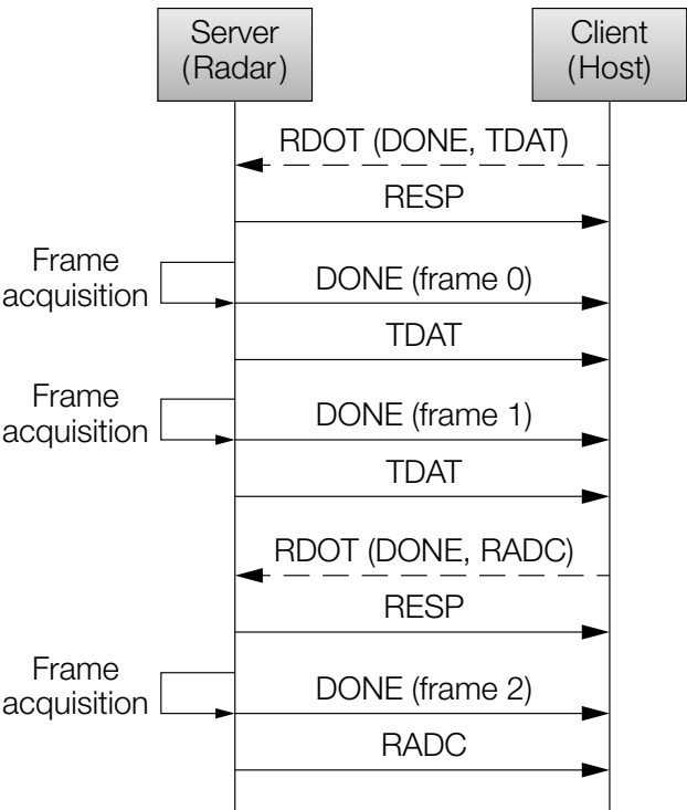
Figure 23: Data output messages
