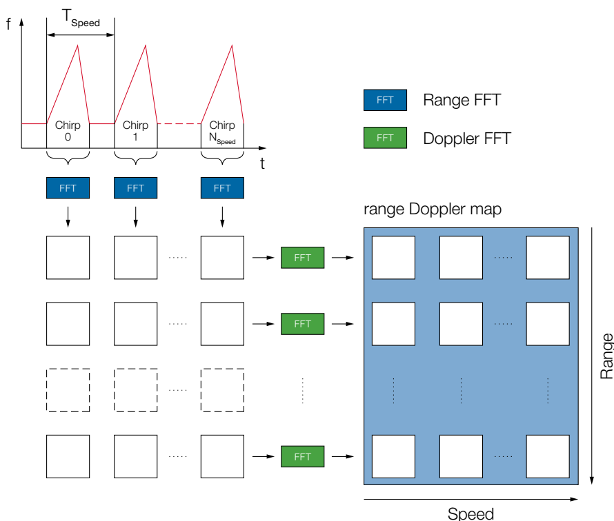
Figure 6: Range Doppler map processing
