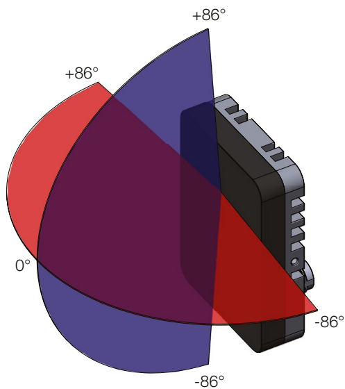
Figure 8: Azimuth and elevation valid angle definition
