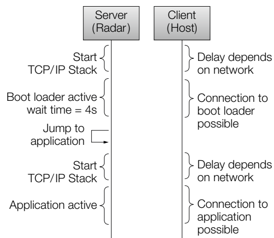
Figure 22: Start-up with connection to boot loader and firmware update
