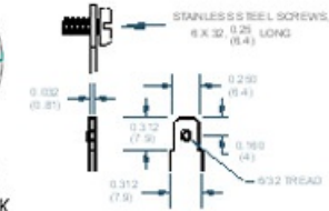
"S" TERMINALS
