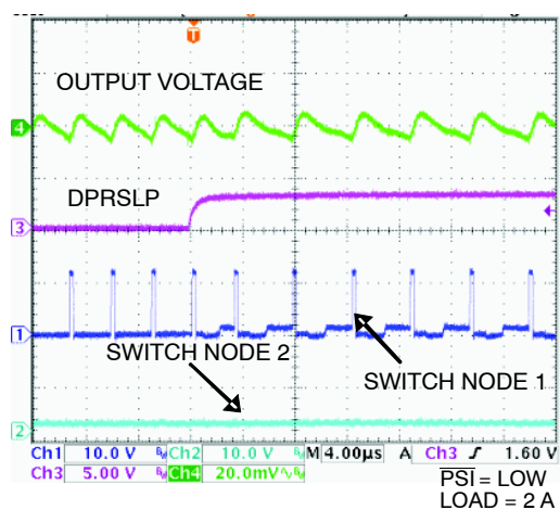
Figure 25. DPRSLP Transition
