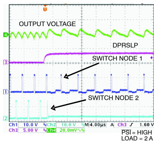
Figure 23. DPRSLP Transition
