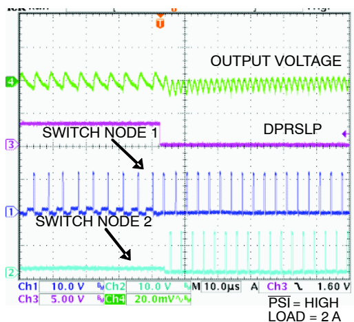
Figure 22. DPRSLP Transition
