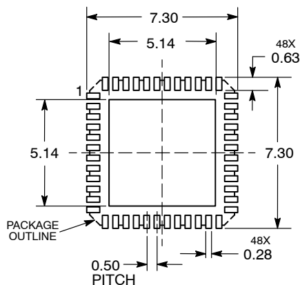
SOLDERING FOOTPRINT*
