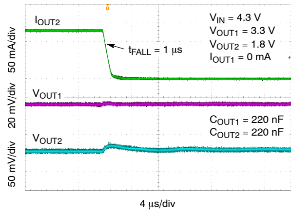
Figure 36. Load Transient Response – Falling Edge, I_{OUT} = 130 \text{ mA} to 1 \text{ mA} – 1.8 \text{ V}
