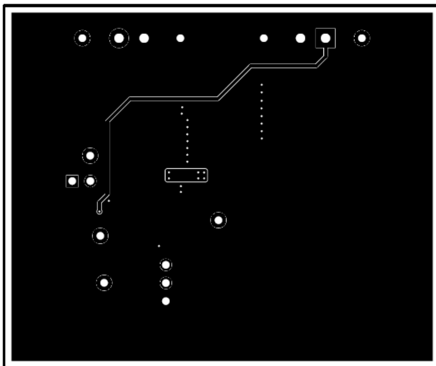
Figure 5-3. Bottom Layer
