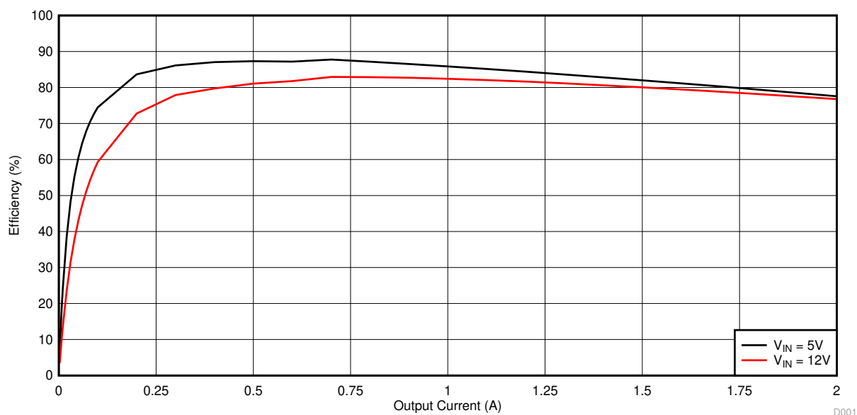
Figure 4-1. TPS562210AEVM-663 Efficiency
