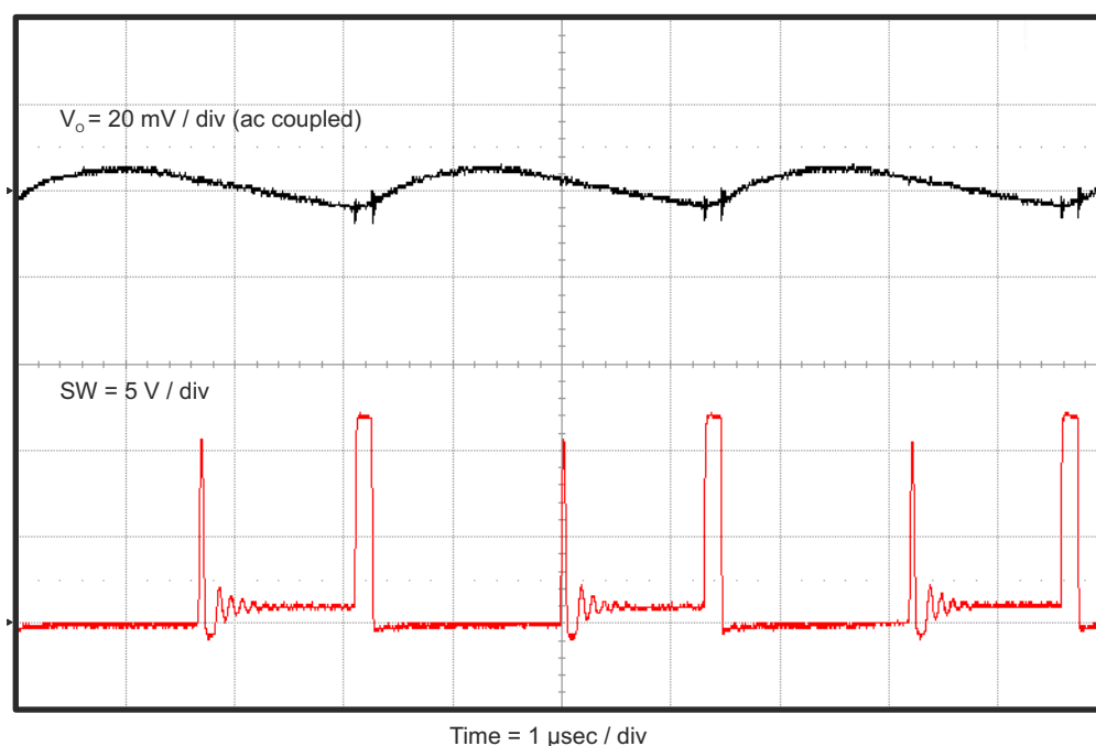
Figure 4-8. TPS562210AEVM-663 Output Voltage Ripple, I_{OUT} = 200 mA
