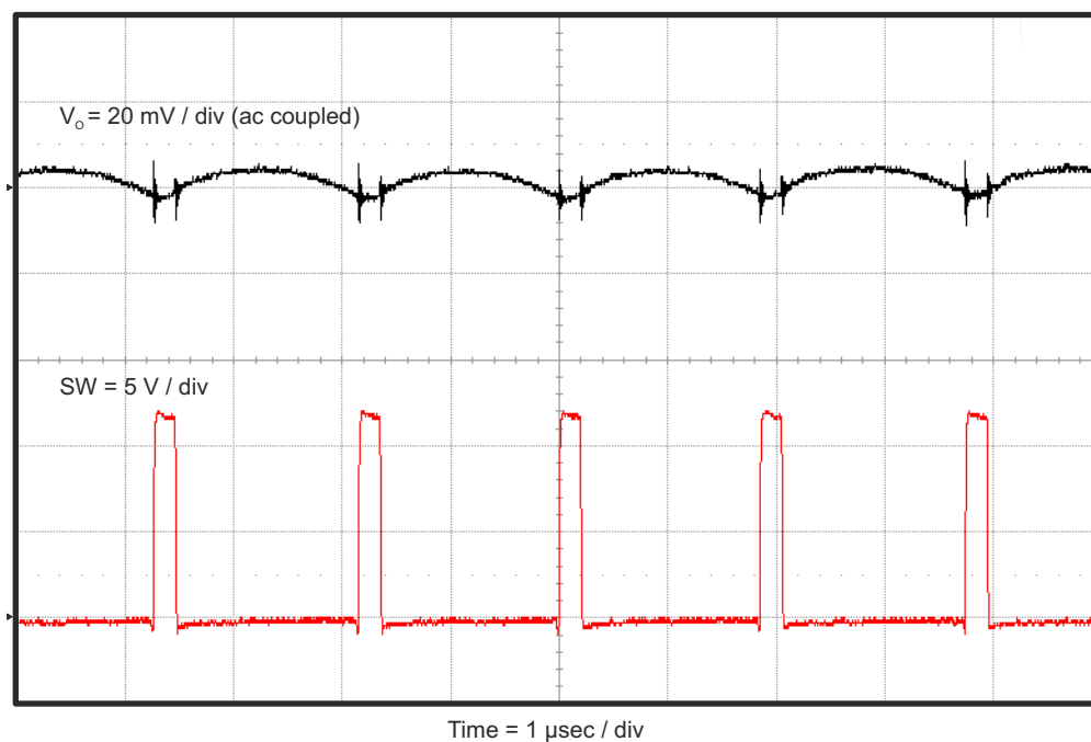
Figure 4-7. TPS562210AEVM-663 Output Voltage Ripple, I_{OUT} = 2 A
