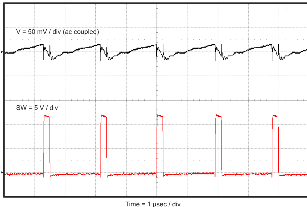
Figure 4-10. TPS562210AEVM-663 Input Voltage Ripple, I_{OUT} = 2 A
