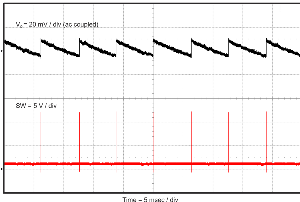
Figure 4-9. TPS562210AEVM-663 Output Voltage Ripple, I_{OUT} = 0 mA
