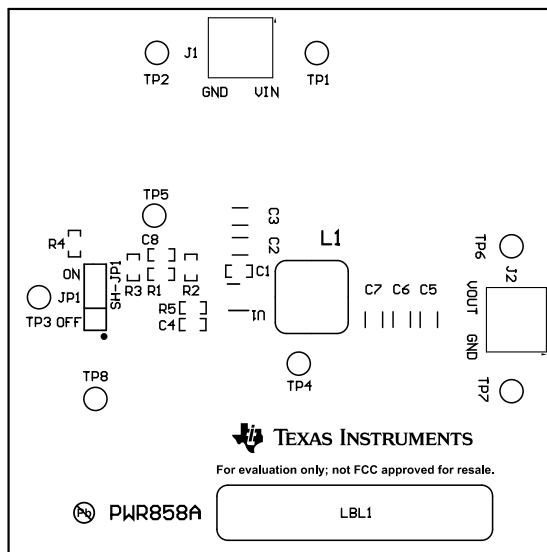
Figure 5-1. Top Assembly
