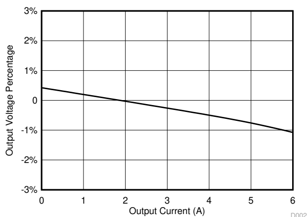
Figure 4-2. Load Regulation
