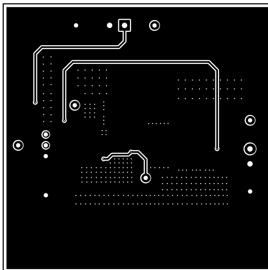
Figure 5-3. Bottom Layer
