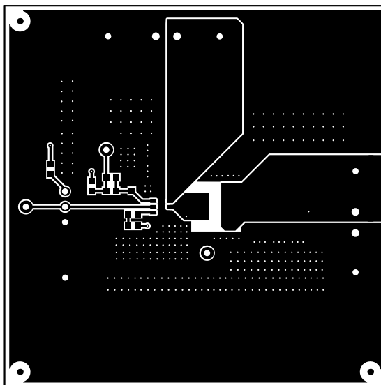
Figure 5-2. Top Layer
