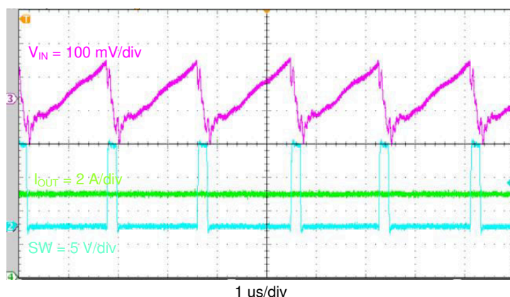
Figure 4-8. TPS565208 Input Voltage Ripple
