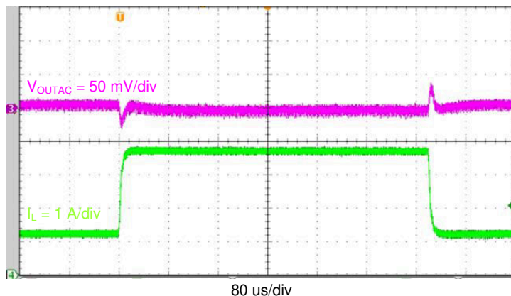
Figure 4-4. TPS565208 Transient Response, 1.25 A to 3.75 A
