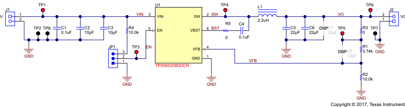
Figure 6-1. TPS565208EVM-858 Schematic Diagram
