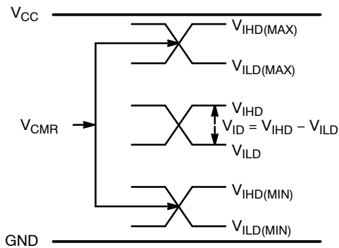
Figure 13. V_{CM} Diagram
