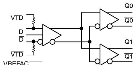
Figure 1. Simplified Logic Diagram
