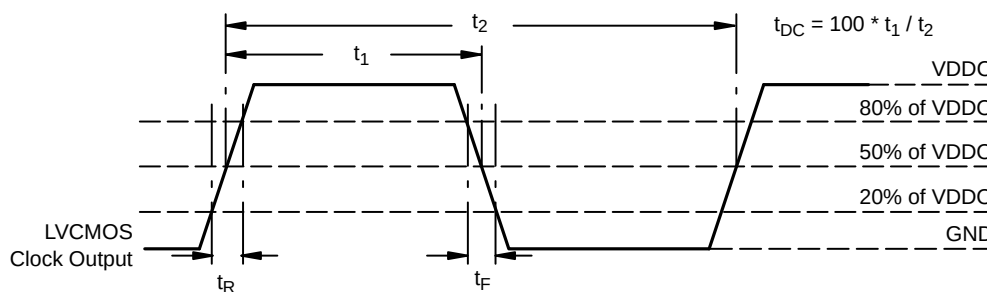
Figure 12. LVC MOS Measurement for AC Parameters
