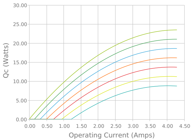
Heat Pumped at Cold Side T_{\text{hot}} = 85^\circ\text{C}
