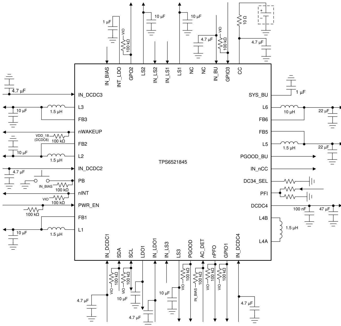
Figure 3-1. Simplified Schematic
