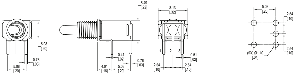
H = Horizontal mount, right angle PC pins, single pole, single throw
