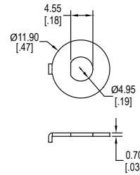
Locking Ring (Flat)
