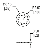
Lock Washer
