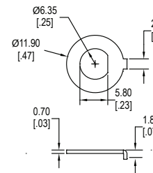
Locking Ring (Flat)
