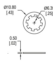
Lock Washer
