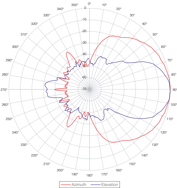
Figure 2: Antenna system diagram (logarithmic scale)
