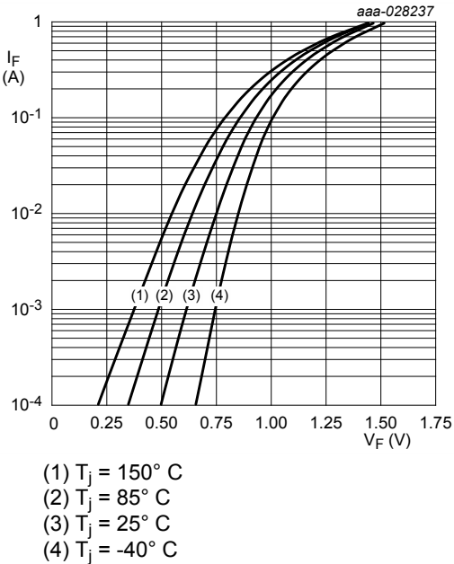
Fig. 5. Forward current as a function of forward voltage; typical values; (logarithmic scale)
