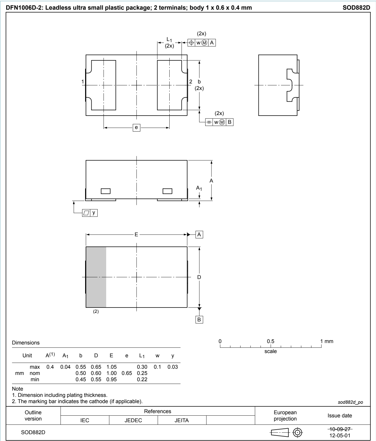
Fig. 10. Package outline DFN1006D-2 (SOD882D)
