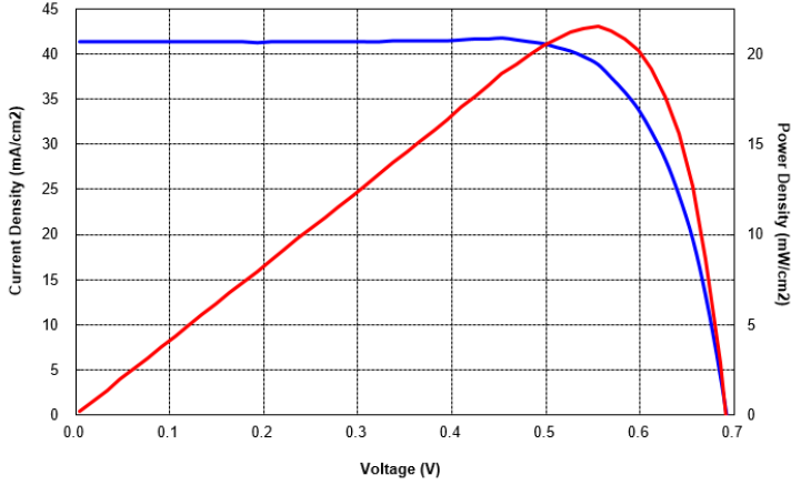
Current-Voltage Characteristics
