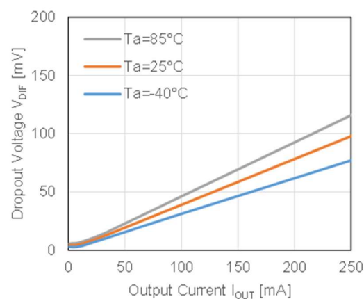
RP123K/N281x
