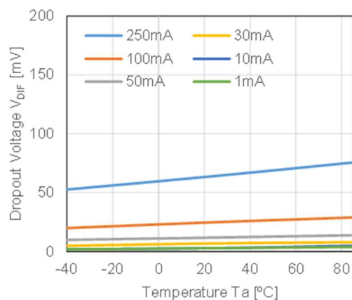
RP123Z48xx
