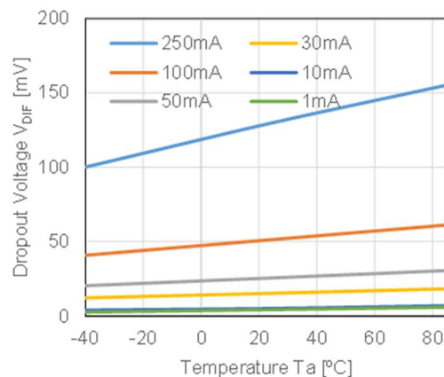
RP123K/N281x
