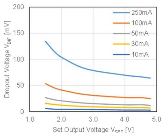
RP123Zxxxx
