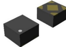
DFN(PLP)1010-4 1.0 x 1.0 x 0.6 (mm)
