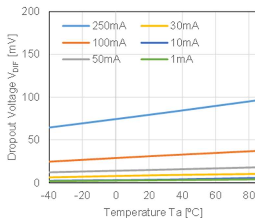
RP123K/N481x
