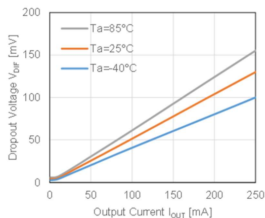
RP123K/N181x
