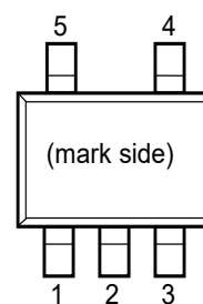
RP123N (SOT-23-5) Pin Configuration
