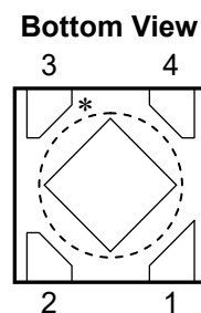
RP123K (DFN(PLP)1010-4) Pin Configuration
