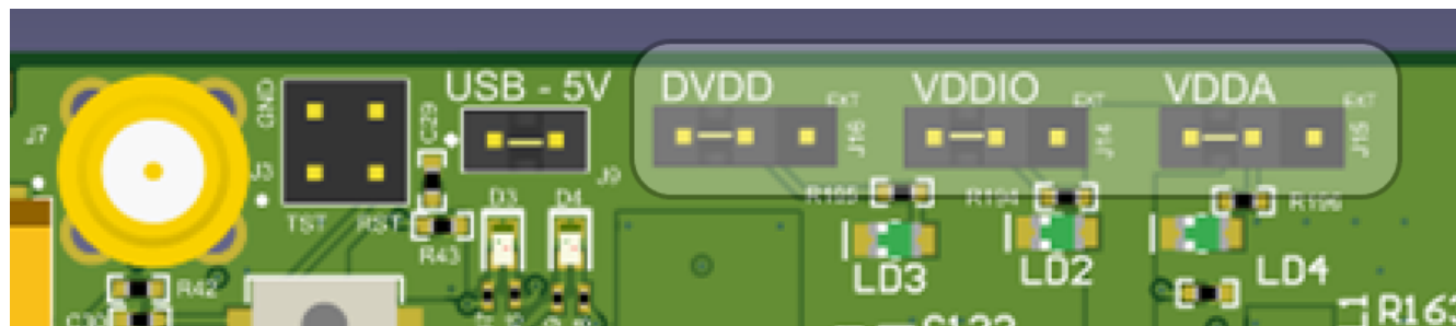
Figure 2-5. DP83TD510E External Supply Connection and Jumpers
