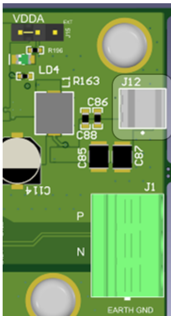
• Place shunt at J14 header in the "On-Board" position to connect VDDIO LDO • Place shunt at J15 header in the "On-Board" position to connect VDDA LDO • Place shunt at J16 header in the "On-Board" position to connect DVDD LDO • Remove Shunt at J9 header • Connect J11 to J25 for Media Converter operation • Wide Vin: Connect 36-V to 5-V to pin 1 of J12 and ground to pin 2 of J12
