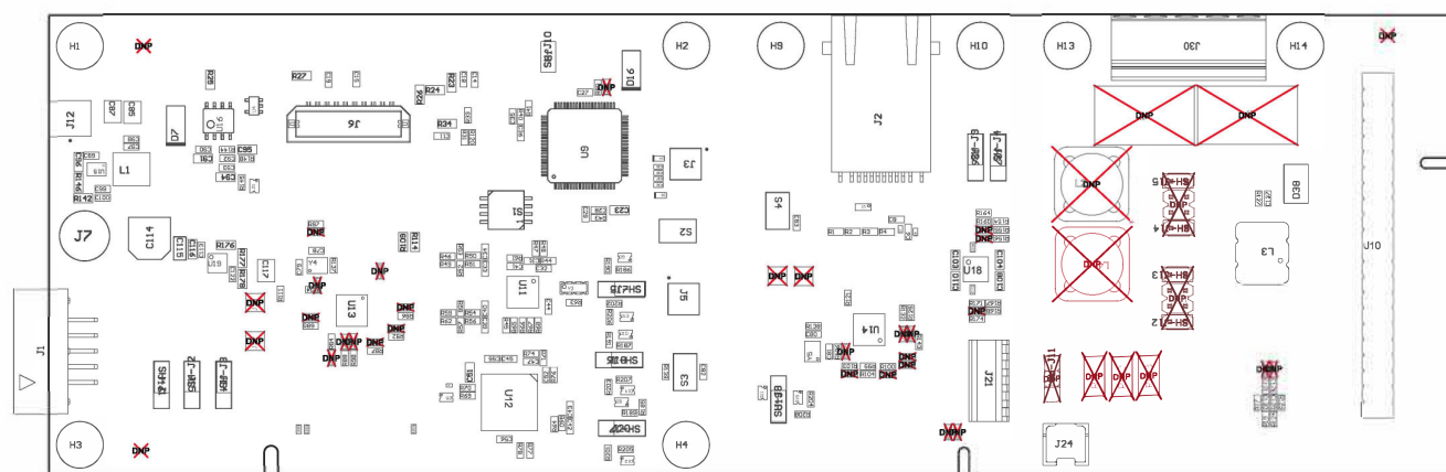
Figure 6-11. Top Assembly
