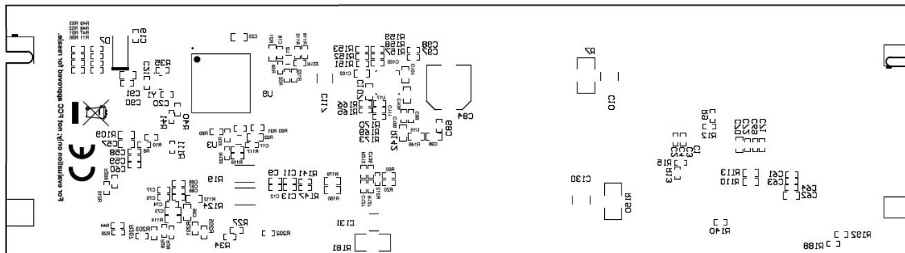
Figure 6-10. Bottom Overlay
