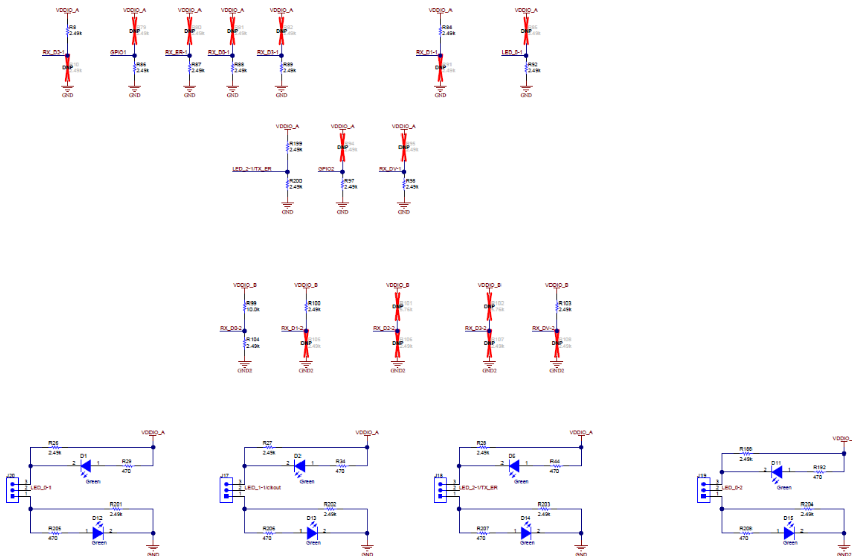
Figure 5-3. DP83TD510E-EVM Interface
