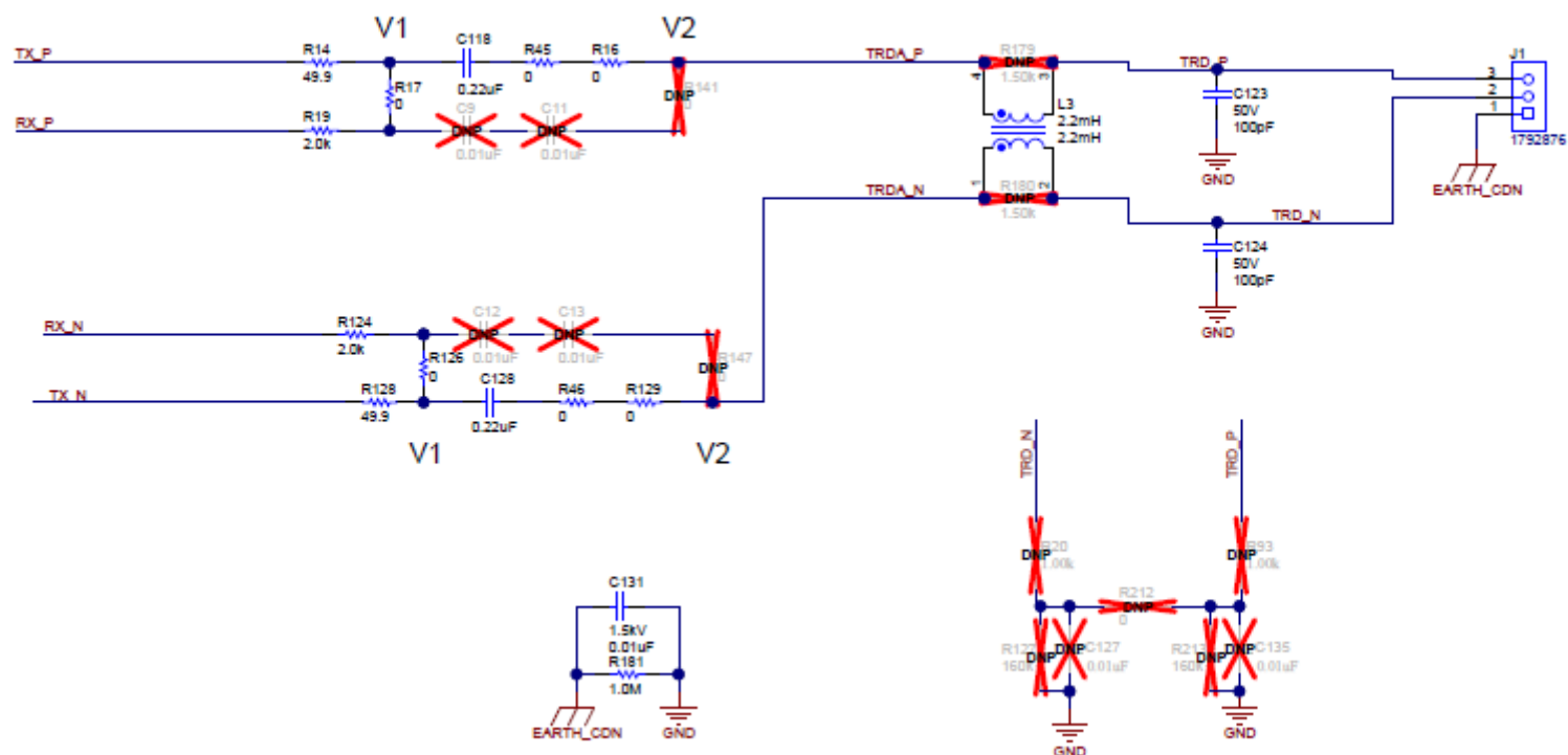
Figure 5-4. DP83TD510E-EVM AFE
