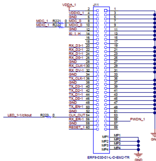
Figure 5-7. DP83TD510E-EVM break-out connector
