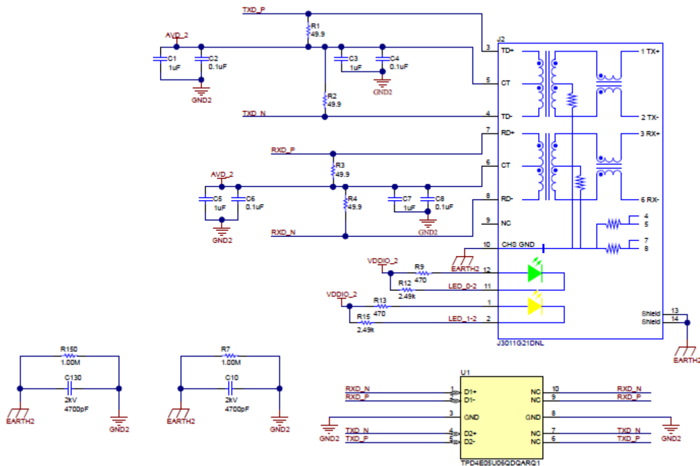
Figure 5-5. DP83822I Media Converter AFE
