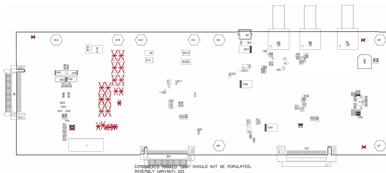
Figure 6-12. Bottom Assembly
