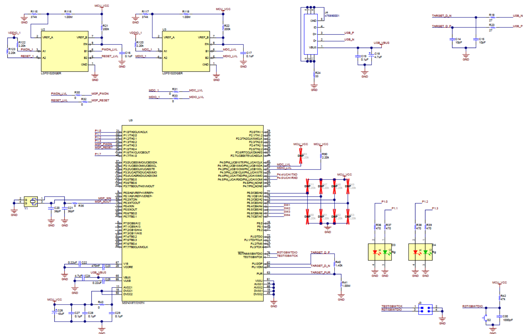
Figure 5-6. DP83TD510E-EVM COMs
