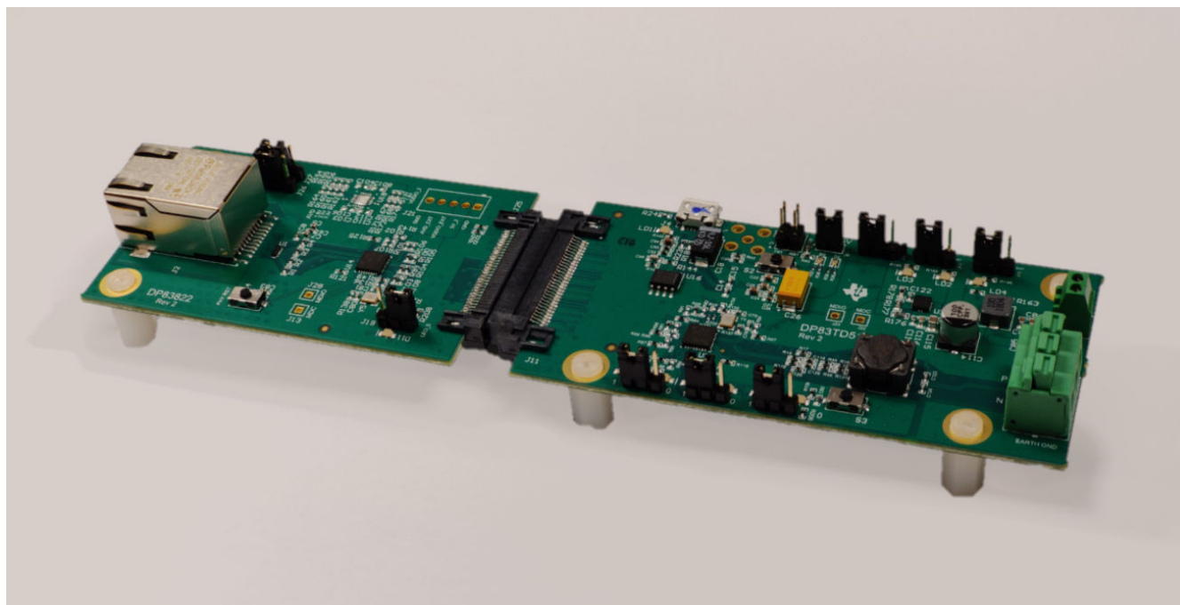
Figure 1-1. DP83TD510E-EVM consists of two PCB's: DP83TD510E Single-Pair-Ethernet board and DP83822I Media-Converter board
