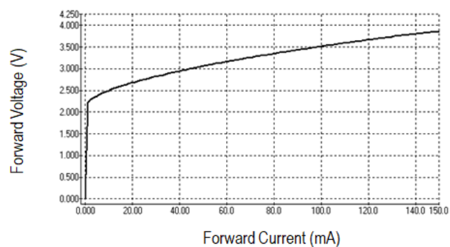
Forward Current vs. Forward Voltage (True Green)
