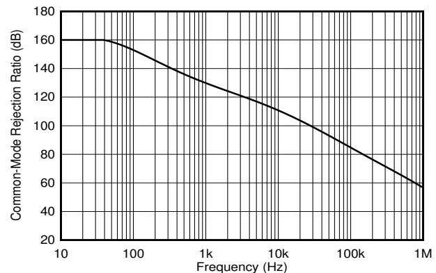
Figure 6-8. Common-Mode Rejection Ratio vs Frequency
