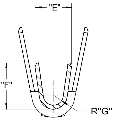
SECTION H-H
