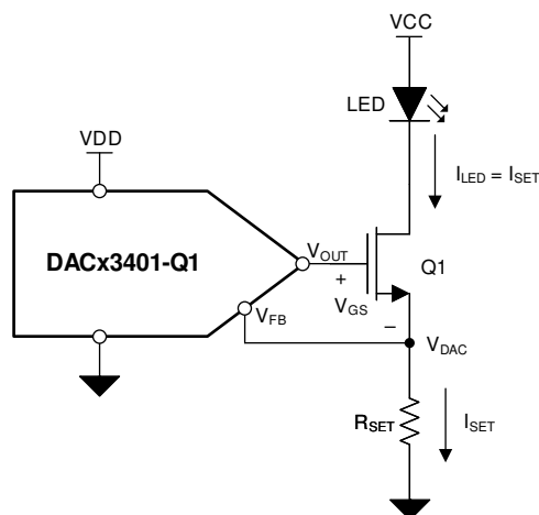
Figure 9-1. LED Biasing
