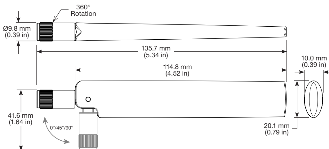
Figure 1. ANT-5GWS1-SMA Antenna Dimensions
