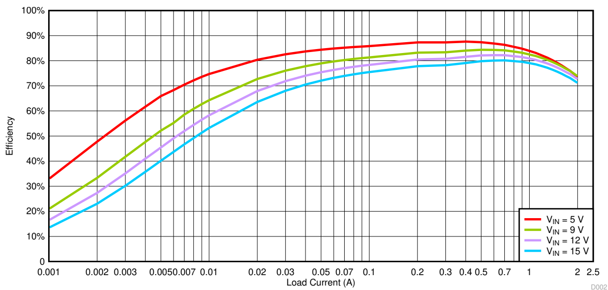
Figure 4-2. Light-Load Efficiency
