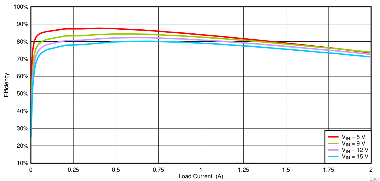
Figure 4-1. Efficiency
