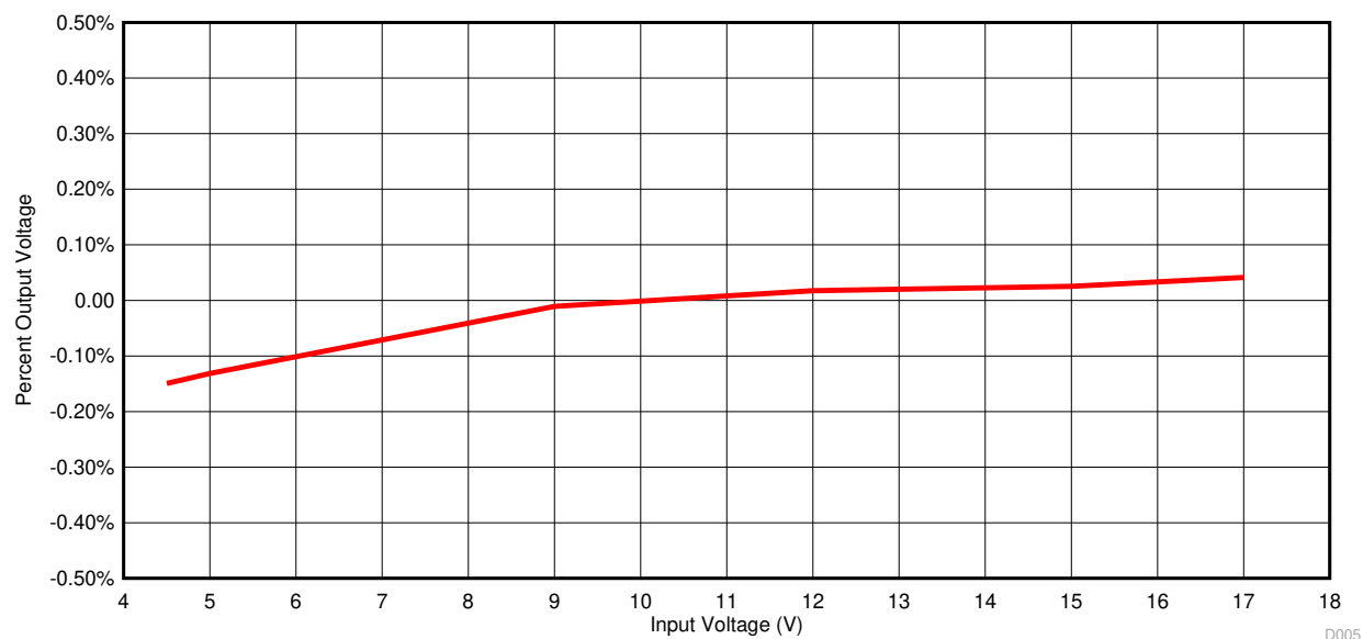
Figure 4-4. Line Regulation
