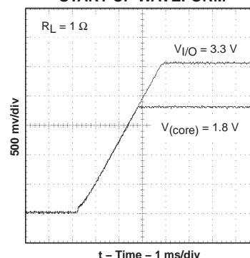
START-UP WAVEFORM
