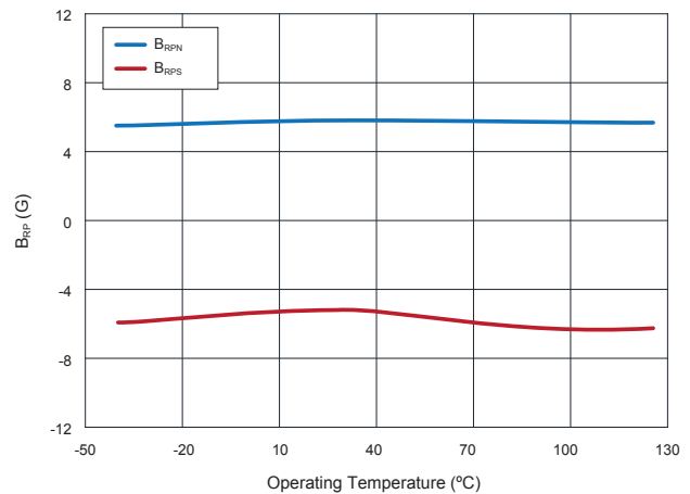
14.7 RR122-1A22-511 / 512 B_{RPN} (Blue) and B_{RPS} (Red) vs. Operating Temperature at V_{DD}=3.0 V
