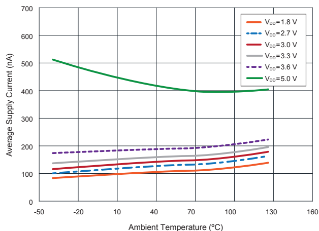
14.2 RR122-1A22-511 / 512 Average Supply Current vs. Temperature vs. Supply Voltage
