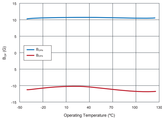
14.6 RR122-1A22-511 / 512 B_{OPN} (Blue) and B_{OPS} (Red) vs. Operating Temperature at V_{DD}=3.0 V
