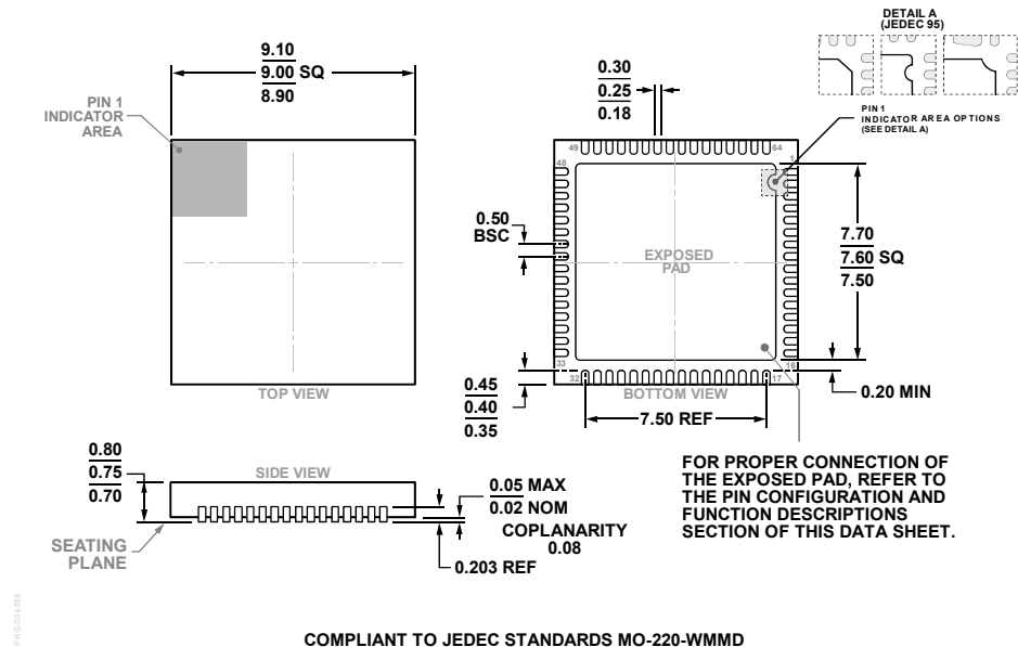
Figure 124. 64-Lead Lead Frame Chip Scale Package [LFCSP] 9 mm × 9 mm Body and 0.75 mm Package Height (CP-64-15) Dimensions shown in millimeters
