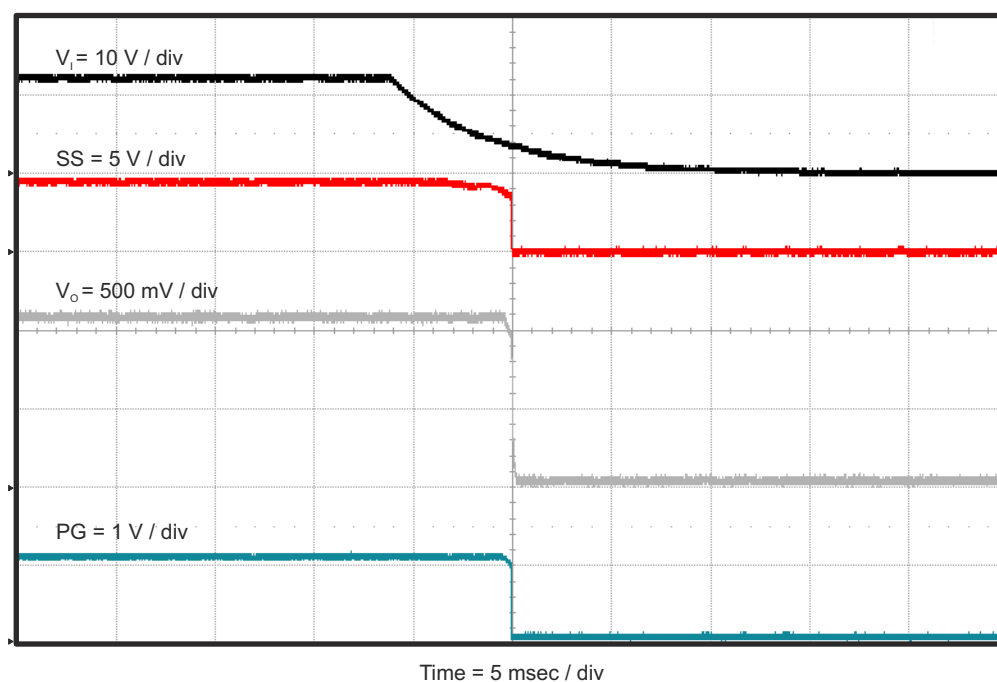
Figure 4-11. TPS562219EVM-663 Shut-Down Relative to V_{IN}
