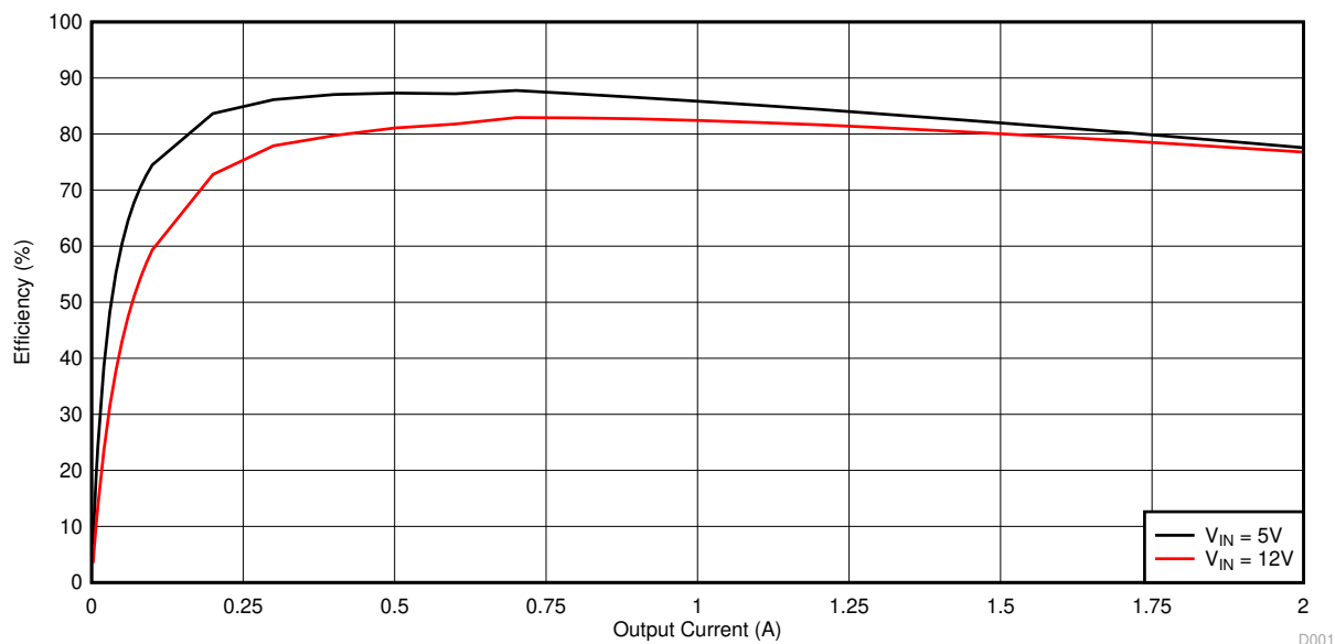
Figure 4-1. TPS562219EVM-663 Efficiency
