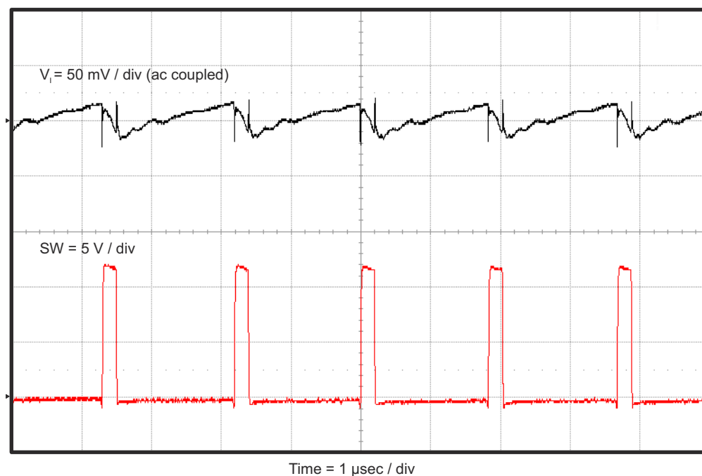
Figure 4-8. TPS562219EVM-663 Input Voltage Ripple, I_{OUT} = 2 A
