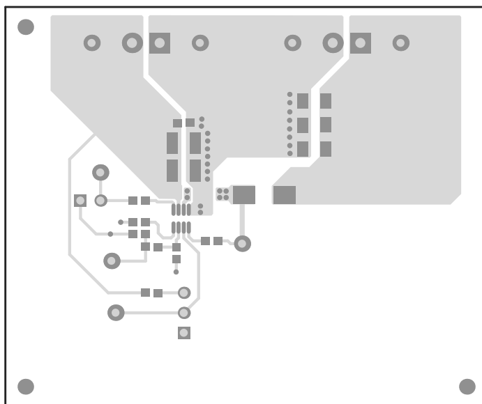
Figure 5-2. Top Layer
