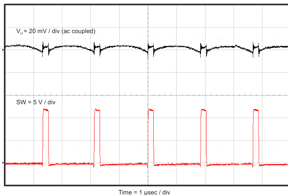
Figure 4-7. TPS562219EVM-663 Output Voltage Ripple, I_{OUT} = 2 A
