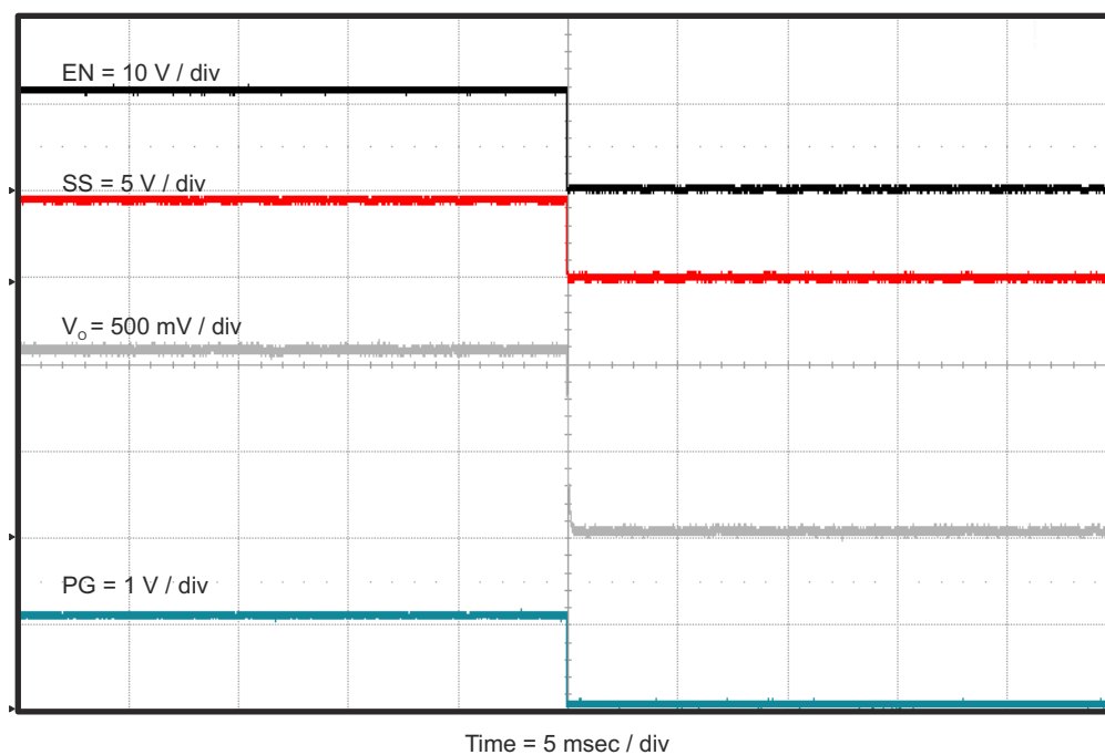
Figure 4-12. TPS562219EVM-663 Shut-Down Relative to EN
