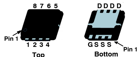
N-Channel MOSFET
