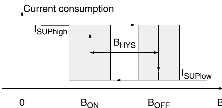
Fig. 4–8: Definition of magnetic switching points for the HAL 1563
