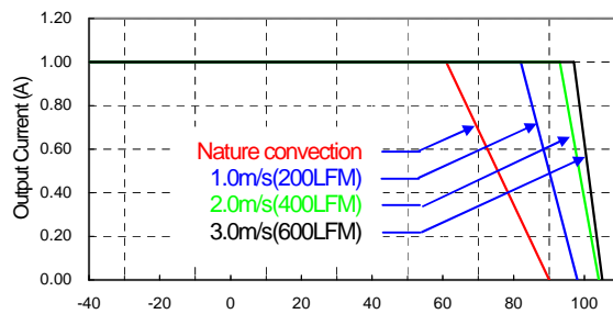
Ambient Temperature, T a (°C) Derating Output Current versus Ambient Temperature and Airflow
