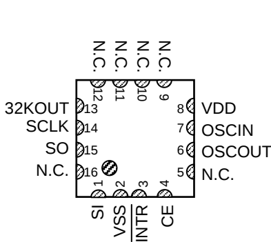
R2043L(QFN023023-16)
