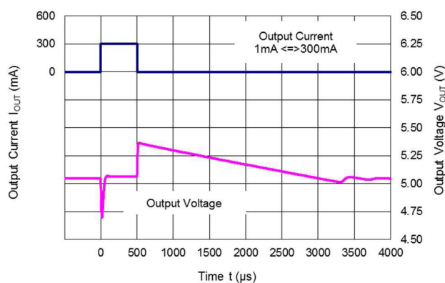
R1518x50xx (C2 = 10 μF)
