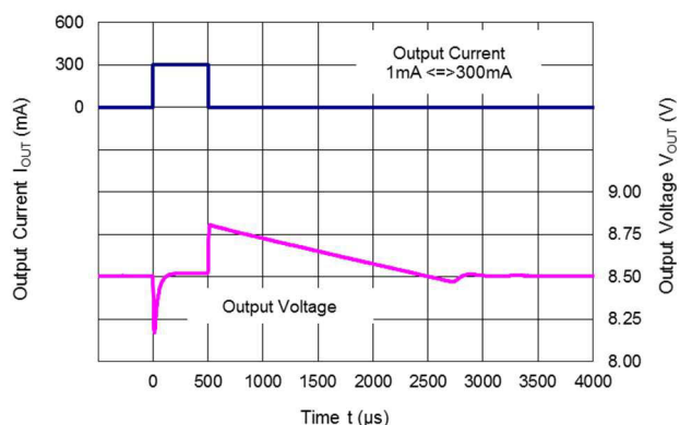
R1518x85xx (C2 = 10 μF)
