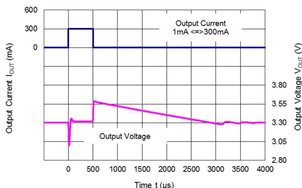
R1518x33xx (C2 = 10 μF)
