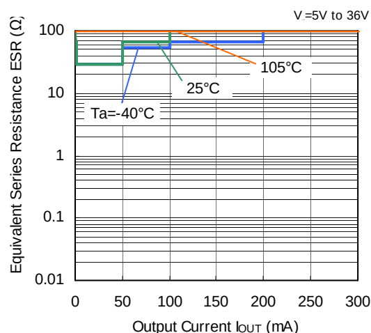
R1511x001C ( V_{OUT}=12\text{V} )
