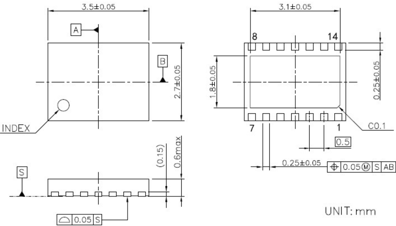
DFN2735-14 Package Dimensions
