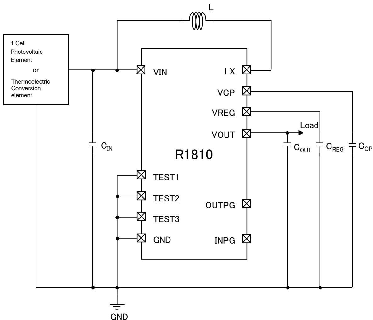
R1810x Typical Application Circuit
