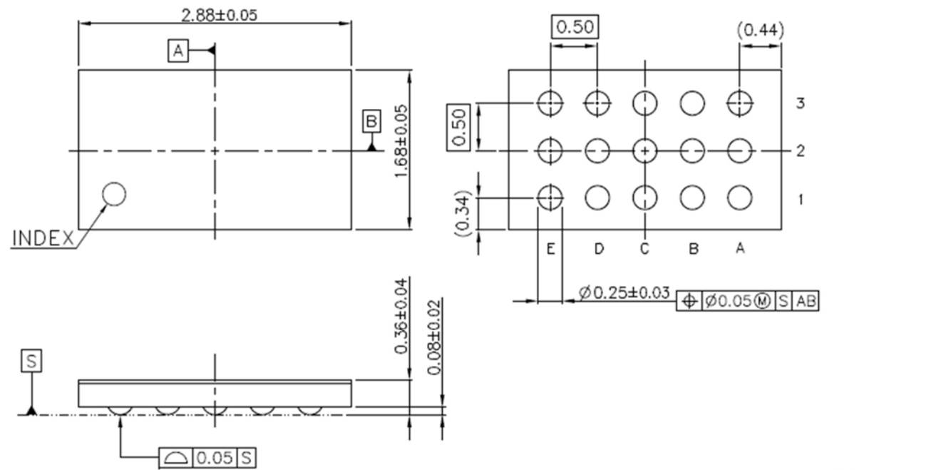
WLCSP-15-P1 Package Dimensions
