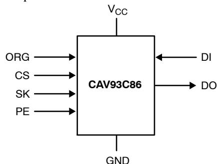
Figure 1. Functional Symbol
