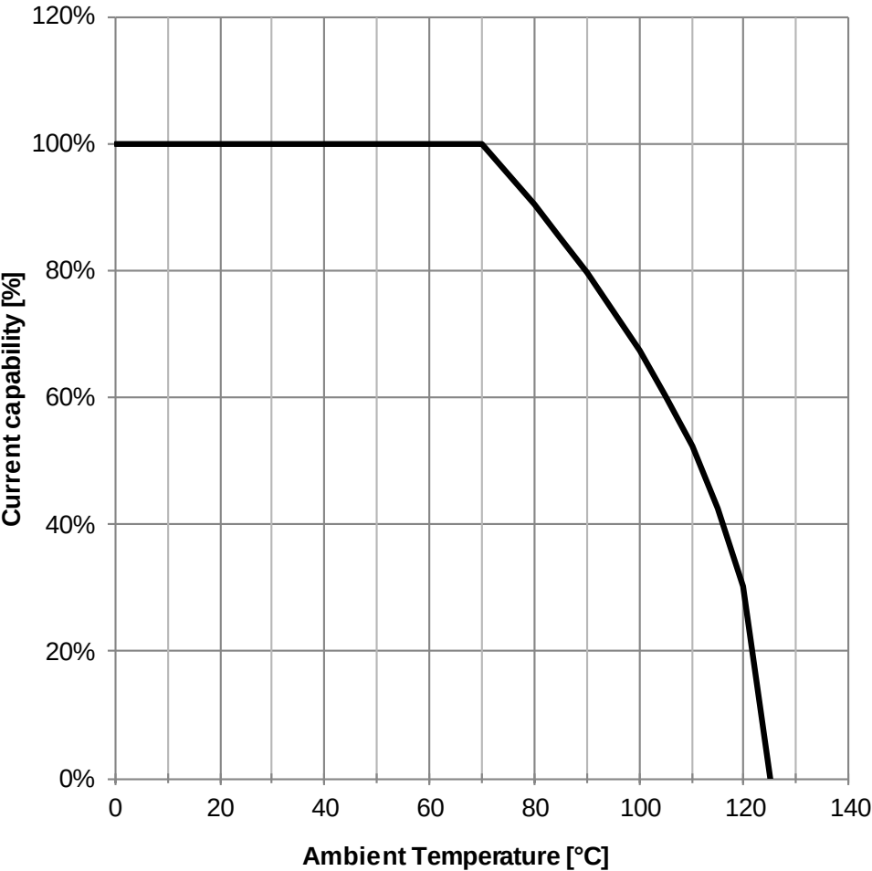
Derating Curve:
