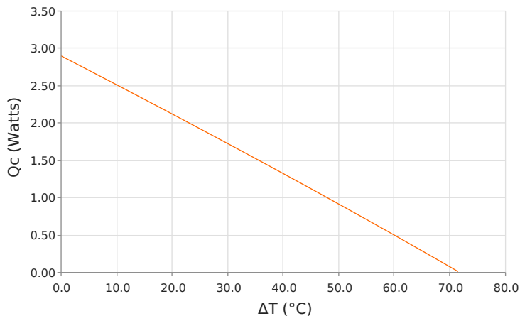
Heat Pumped at Cold Side ( Q_c ) T_{hot} = 27^\circ\text{C} | Current = 1.6 Amps
