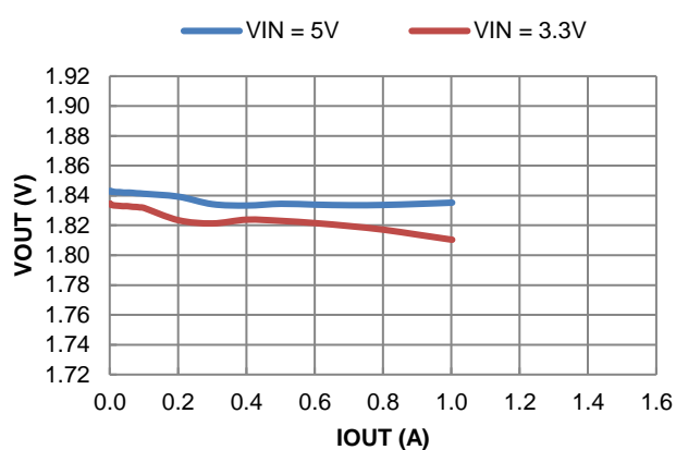
Figure 24. Load Regulation
