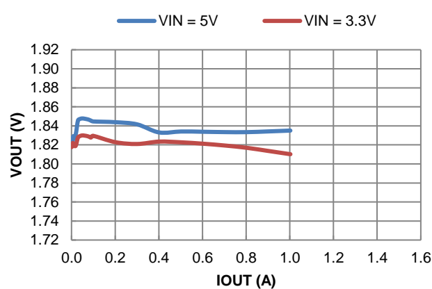
Figure 13. Load Regulation
