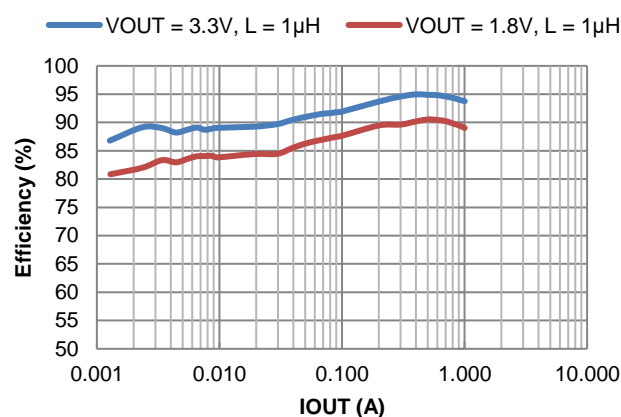
Figure 11. Efficiency vs. Output Current, V_{IN} = 5\text{V}
