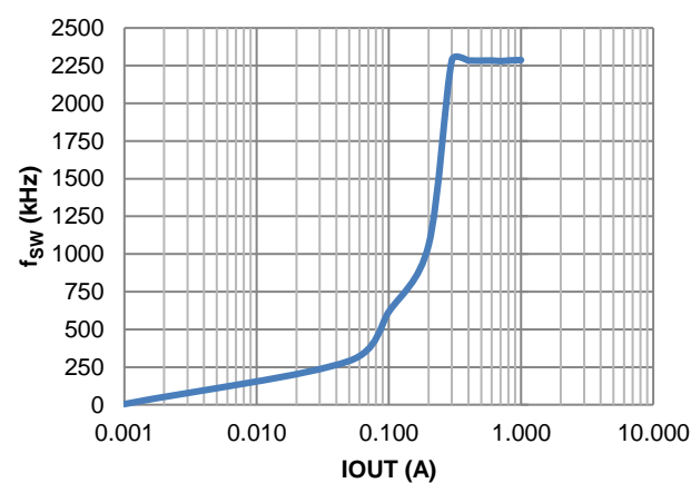
Figure 15. f_{sw} vs. Load
