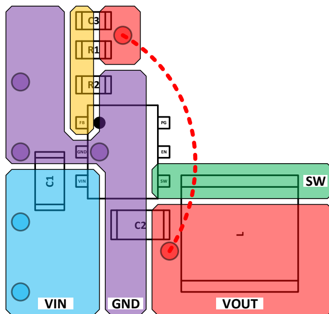
Figure 43. Recommended AP61102 PCB Layout
