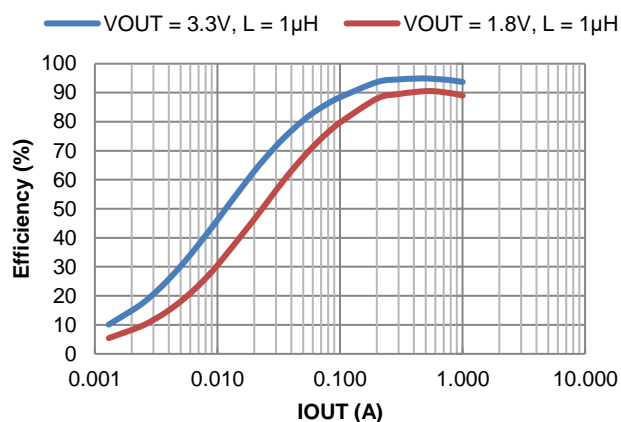
Figure 22. Efficiency vs. Output Current, V_{IN} = 5\text{V}
