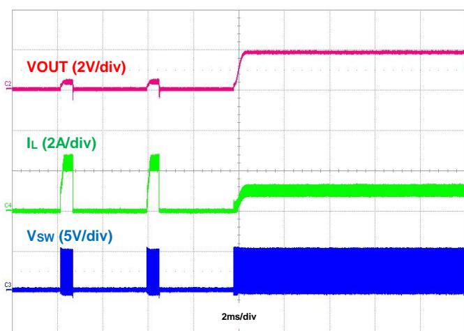
Figure 36. Output Short Recovery, I_{OUT} = 1\text{A}
