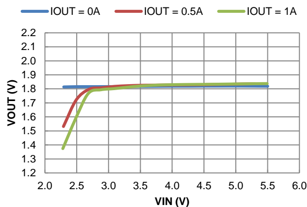
Figure 12. Line Regulation
