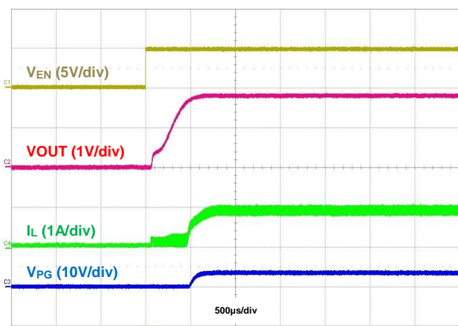
Figure 37. Startup Using EN, I_{OUT} = 1\text{A}
