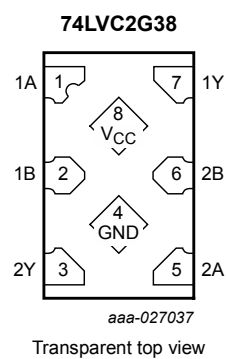
Figure 7. Pin configuration SOT1233
