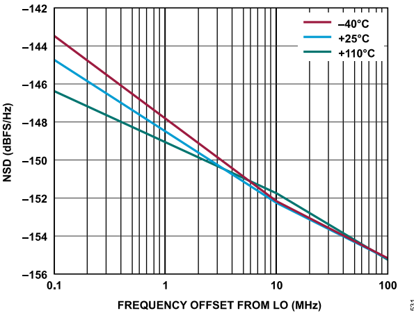
Figure 291. Transmitter NSD vs. Frequency Offset from LO, Baseband Frequency = 2.1 kHz
