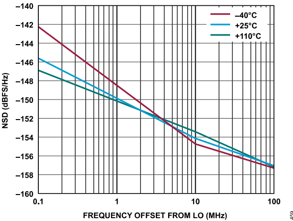
Figure 253. Transmitter NSD vs. Frequency Offset from LO, Baseband Frequency = 2.1 kHz
