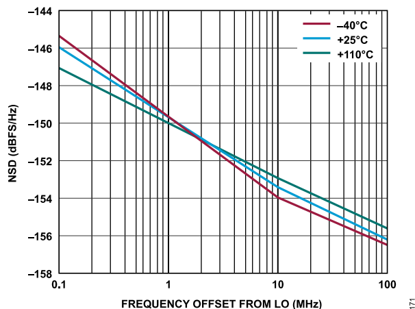
Figure 63. Transmitter NSD vs. Frequency Offset from LO, Baseband Frequency = 5.6 MHz
