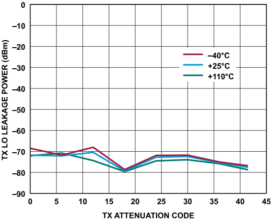
Figure 214. Transmitter LO Leakage Power vs. Transmitter Attenuation Code, Baseband Frequency = 2.1 kHz, Backoff = 6 dBFS, Initialization Calibration Only
