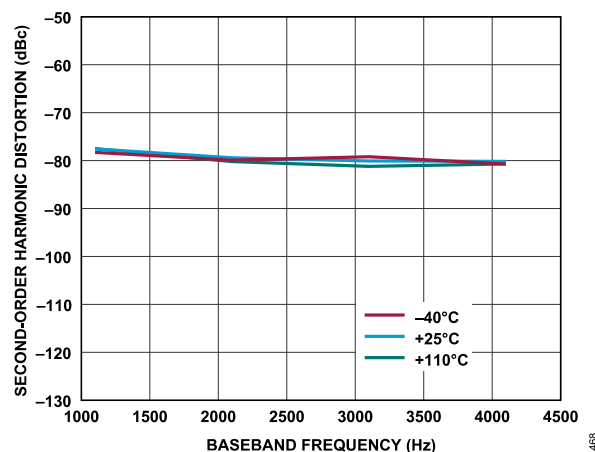
Figure 258. Receiver Second-Order Harmonic Distortion vs. Baseband Frequency, Gain Index = 255, ADC = High Performance
