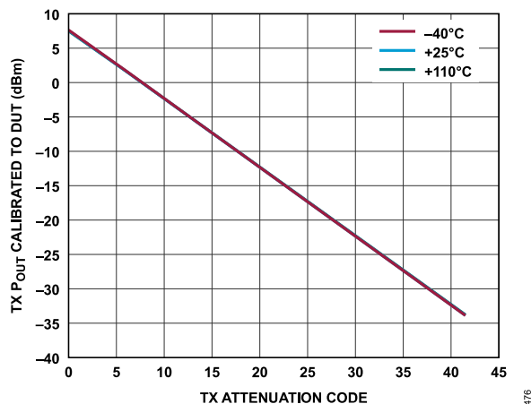
Figure 266. Transmitter Absolute Power vs. Transmitter Attenuation Code, Baseband Frequency = 2.1 kHz, Backoff = 0.2 dBFS
