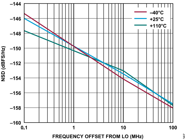
Figure 215. Transmitter NSD vs. Frequency Offset from LO, Baseband Frequency = 2.1 kHz
