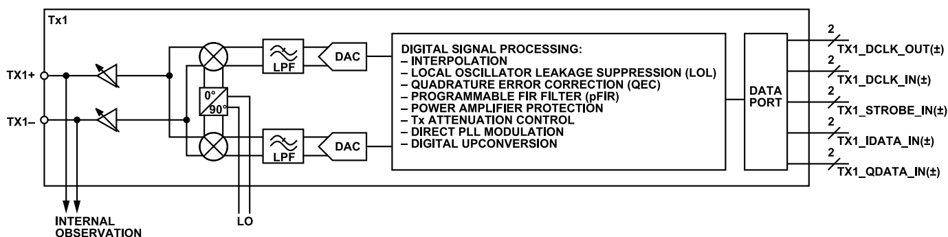
Figure 298. Transmitter Architecture
