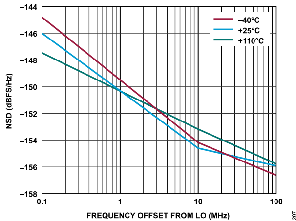
Figure 90. Transmitter NSD vs. Frequency Offset from LO, Baseband Frequency = 5.6 MHz
