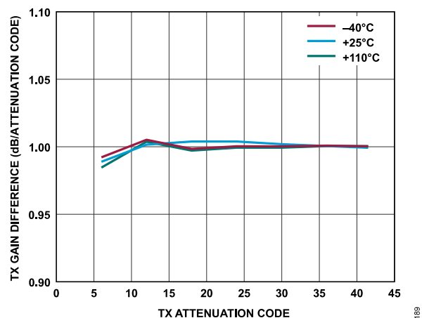
Figure 81. Transmitter Attenuation Delta (Error) vs. Transmitter Attenuation Code, Baseband Frequency = 18 MHz, Backoff = 0.2 dBFS
