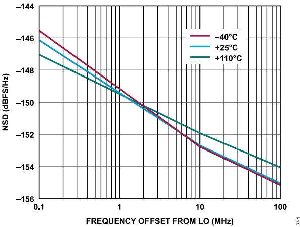
Figure 196. Transmitter NSD vs. Frequency Offset from LO, Baseband Frequency = 2.1 kHz
