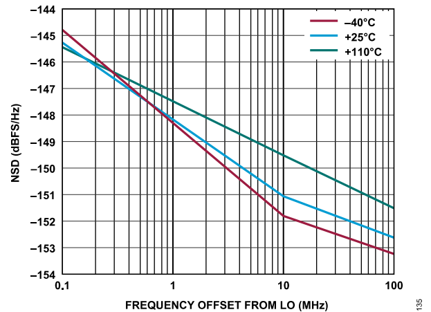
Figure 36. Transmitter NSD vs. Frequency Offset from LO, Baseband Frequency = 5.6 MHz
