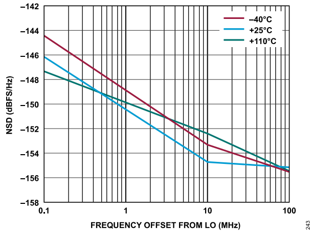
Figure 117. Transmitter NSD vs. Frequency Offset from LO, Baseband Frequency = 5.6 MHz
