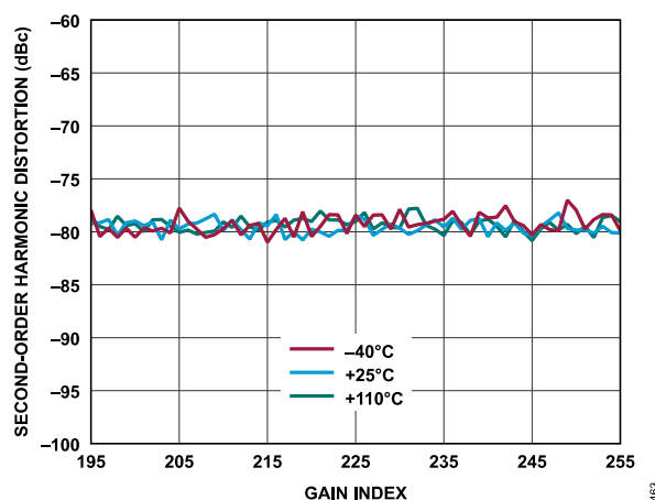
Figure 257. Receiver Second-Order Harmonic Distortion vs. Gain Index, Baseband Frequency = 2.1 kHz, ADC = High Performance
