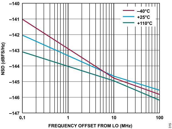
Figure 177. Transmitter NSD vs. Frequency Offset from LO, Baseband Frequency = 5.6 MHz
