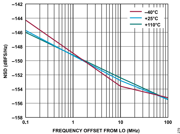
Figure 150. Transmitter NSD vs. Frequency Offset from LO, Baseband Frequency = 5.6 MHz
