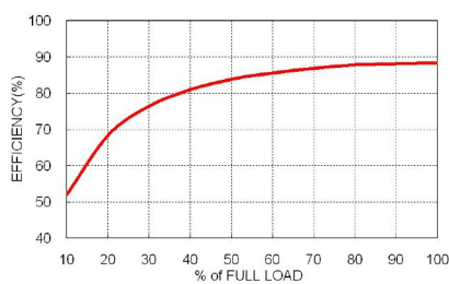
FED30-48S05W Efficiency vs. Output Load
