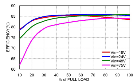
MPP10-48S05WA Efficiency vs. Output Load
