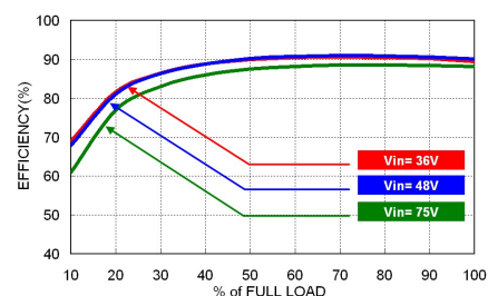
DFEC40-48S05 Efficiency vs. Output Load
