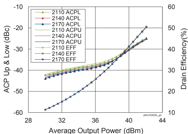
Single-carrier WCDMA 3GPP Drive-up V_{DD} = 28\text{ V} , I_{DQ} = 170\text{ mA} , 3GPP WCDMA signal, PAR = 7.5 dB, BW = 3.84 MHz
