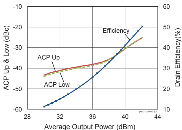
Single-carrier WCDMA Drive-up V_{DD} = 28\text{ V} , I_{DQ} = 170\text{ mA} , f = 2170\text{ MHz} , 3GPP WCDMA signal, PAR = 7.5 dB, BW = 3.84 MHz
