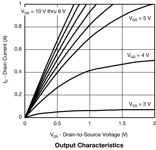
Output Characteristics
