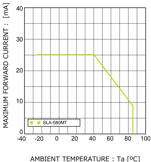
Fig.4 Derating
